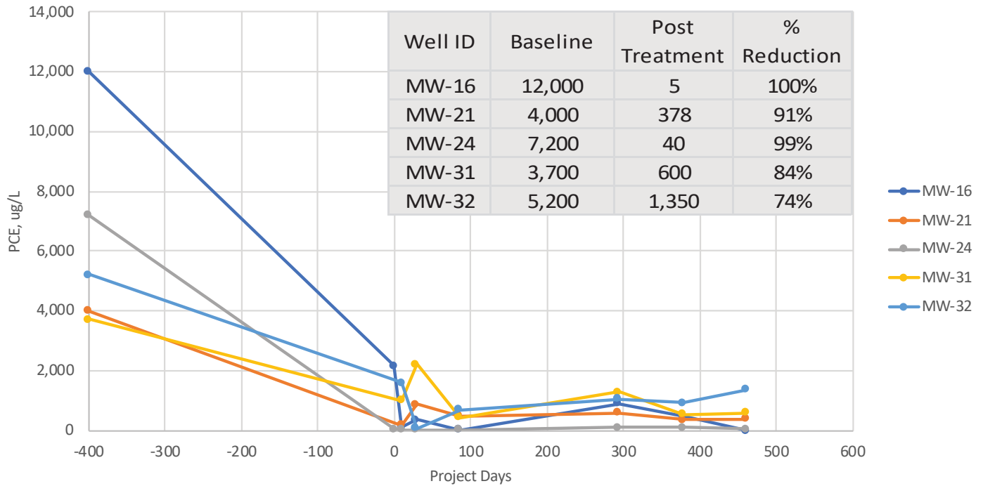
Figure 2. PCE Concentrations versus Time
